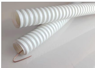
Photo. 2 RKSGHF of PC/ABS 750 N without and with guide wire
